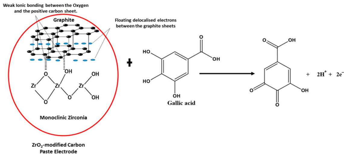
Fig. 14 Proposed interaction between \text{ZrO}_2 NPs and graphite, demonstrating a weak ionic bond between some of the oxygen and the positive graphite sheet in the electrochemical determination of gallic acid. 133
