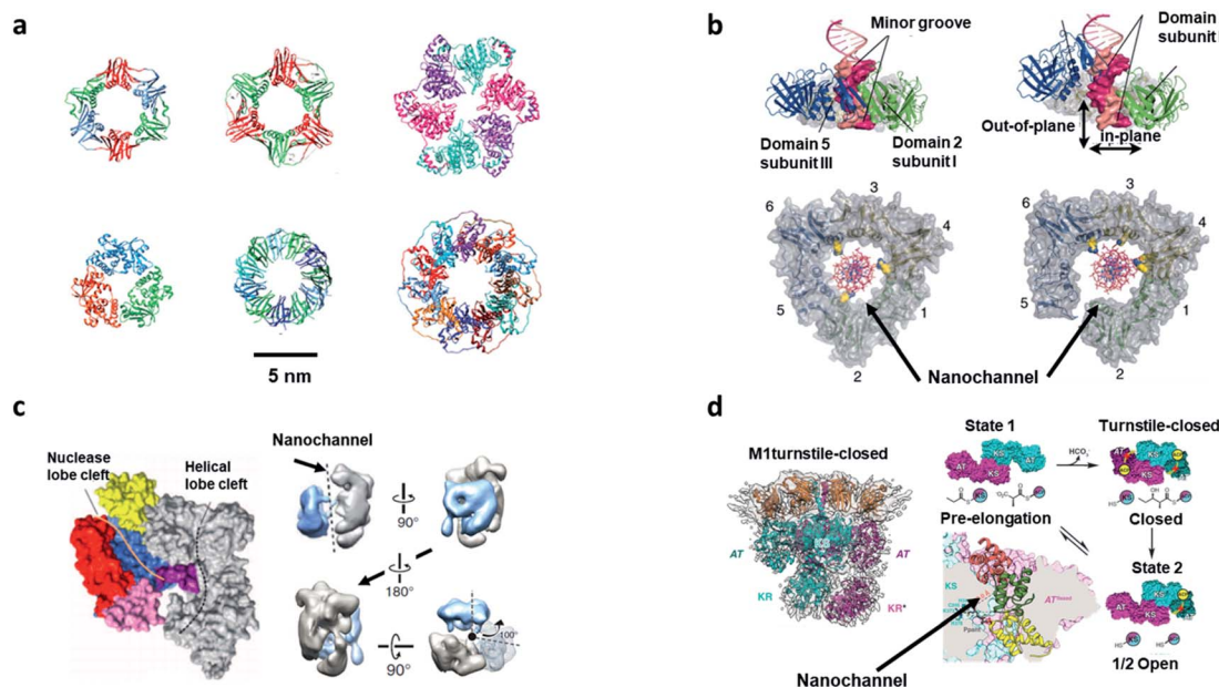
Fig. 3 Biological reactions with CCE in bio-nanochannels. (a) Ring proteins in different species. First line: the \beta -clamp of E. coli (PDB: 2POL), the proliferating cell nuclear antigen of H. sapiens (PDB: 1AXC), helicase of bacteriophage (PDB: 1QAW). Second line: the exonuclease of bacteriophage (PDB: 1AVQ), RNA binding protein of Bacillus stearothermophilus (PDB: 1QAW), and DNA binding protein of Homo sapiens (PDB: 1KN0). Scale bar: 5 nm. Reproduced from ref. 7 with permission from the Royal Society of Chemistry. (b) The nanochannel of ring-shaped (DNA clamp) encircles the DNA template and allows the DNA polymerases to slide along the DNA strand in an effective and fast way. Reproduced with permission. 52 Copyright 2011, American Association for the Advancement of Science. (c) Left: crystal structure of Cas 9 with nanochannels and nucleic acid binding clefts. Right: rotation view of the structures of Cas 9 (black dashed line represents the central channel). Reproduced with permission. 54 Copyright 2014, American Association for the Advancement of Science. (d) Structure of DEBS M1 and the turnstile-closed/opened state. Left: the structure of DEBS M1 by cryogenic electron microscopy (4.3 Å-resolution). Right: three states of the DEBS M1. State 1 (pre-elongation) with the accessibility of the AT and KS active site. Then, the proteins undergo a conformational change to a turnstile-closed state with the inaccessibility of the AT and KS. After that, acyl carrier proteins are hindered by the KS active site but have access to the AT active site. Reproduced with permission. 57 Copyright 2021, American Association for the Advancement of Science.
