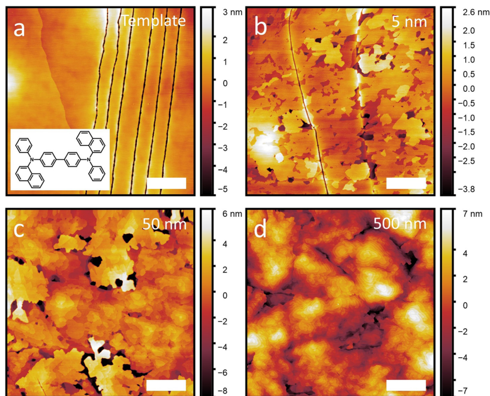
Fig. 1 Atomic force microscope images of an (a) NPB template crystal and (b) 5 nm, (c) 50 nm and (d) 500 nm of additional NPB grown on top of the template. Scale bars are 1 μm. Molecular structure of NPB is shown as an inset in (a).
