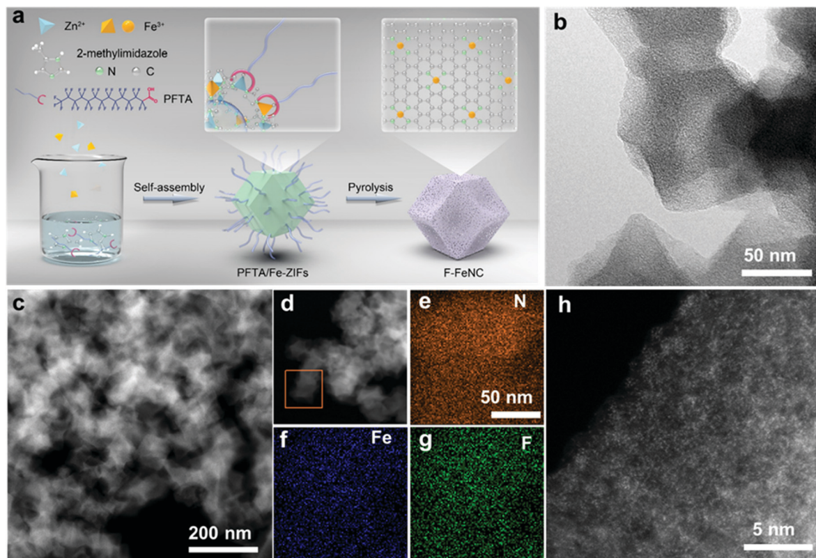
Fig. 1 (a) Illustration of the synthesis of F-FeNC catalysts. (b) TEM and (c) and (d) STEM of the obtained F-FeNC-2 catalyst. Elemental mapping of (e) N, (f) Fe, and (g) F of the highlighted area in (d). (h) Aberration-corrected HAADF-STEM image of F-FeNC-2.
