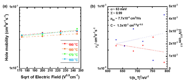
Fig. 7 (a) Hole mobilities plotted for the square root of the electric field at various temperatures in the N* phase of the compounds 1–3 mixture (high temperature region). (b) Plots of zero-field mobility \mu_0 and \beta as a function of the square of 1/k_B T in the N* phase of the LC mixture (high temperature region).
