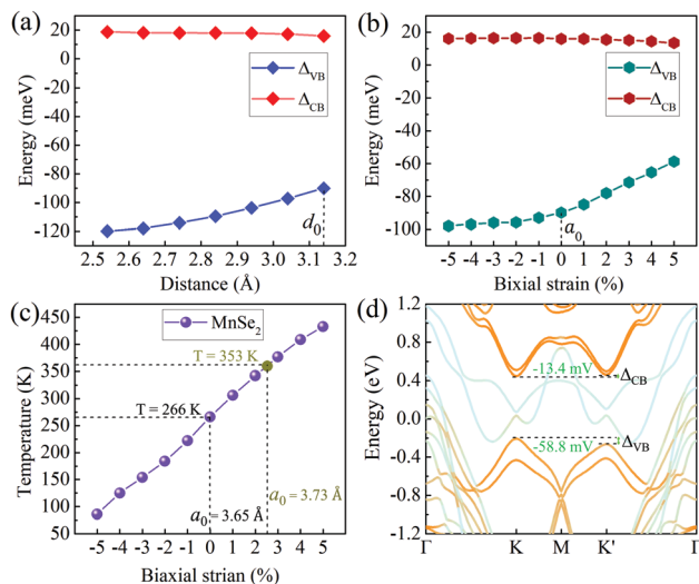
Fig. 4 (a and b) valley-splitting changes versus interlayer distance and biaxial strain, respectively. (c) Curie temperatures changes versus biaxial strain of monolayer \text{MnSe}_2 . (d) Band structure of \text{MoTe}_2/\text{MnSe}_2 under 5% tensile strain.
