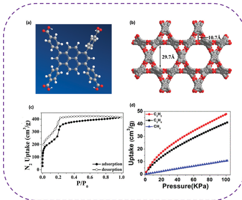
Fig. 8 (a) To construct the molecular structure of PFC-2. (b) The porous frame structure of PFC-2 and two kinds of channels. (c) N_2 adsorption–desorption isotherms (77 K) of desolvated PFC-2. (d) \text{CH}_4 , \text{C}_2\text{H}_2 , and \text{C}_2\text{H}_4 single component adsorption isotherm of PFC-2 at 298 K. Reproduced from ref. 40. Copyright 2019 American Chemical Society.
