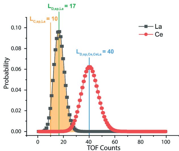
Fig. 6 Detection limits for mm-Ce-La NPs are a function of the critical value of La ( L_{c,sp,La} ) as well as the ratio of Ce:La as controlled by Poisson statistics. Here, the detection limit for a Ce-La NP ( L_{D,sp,Ce,Ce-La} ) is the average Ce signal that leads to 95% ( \beta = 0.05 ) of the La signal distribution to be above L_{c,sp,La} .
