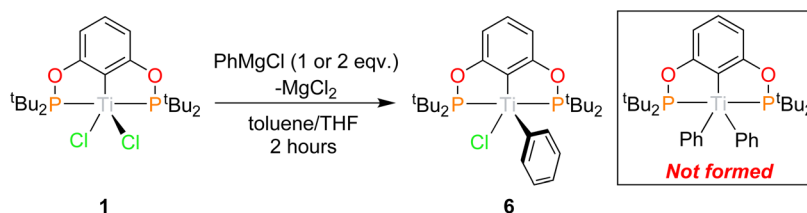
Scheme 7 Synthetic route to (t\text{BuPOCOP})\text{TiPhCl} .
