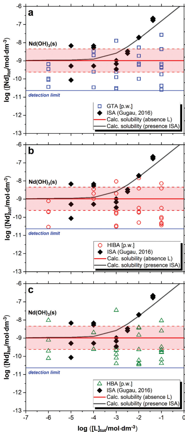
Fig. 4 Solubility of \text{Nd(OH)}_3(\text{s}) in equilibrium with cement porewater at \text{pH} = 12.5 with 10^{-6} \text{ M} \leq [\text{L}]_{\text{tot}} \leq 0.1 \text{ M} at t \leq 358 days: (a) glutaric acid (GTA); (b) \alpha -hydroxyisobutyric acid (HIBA); (c) 3-hydroxybutyric acid (HBA). Red solid and dashed lines in the figure represent the calculated solubility of \text{Nd(OH)}_3(\text{s}) and corresponding uncertainty at \text{pH} = 12.5 in ligand-free systems as reported in Neck et al. , (2009). 20 Black symbols and line correspond to the experimental and calculated solubility of \text{Nd(OH)}_3(\text{s}) in the presence of ISA as reported in Gugau (2016). 61
