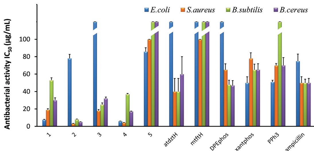
Fig. 3 In vitro antibacterial activity of 1–5 , and their ligands atdztH, mtfH, DPEphos, xantphos, and PPh _3 in free form, expressed as half-minimum inhibitory concentration (IC _{50} ) values ( \mu\text{g mL}^{-1} ) provided by a nonlinear curve fit-growth/sigmoidal-dose response on the experimental optical density data. Values are expressed as mean \pm standard deviation (SD) of three replicate measurements (with the exception of values higher than 100 \mu\text{g mL}^{-1} ).
