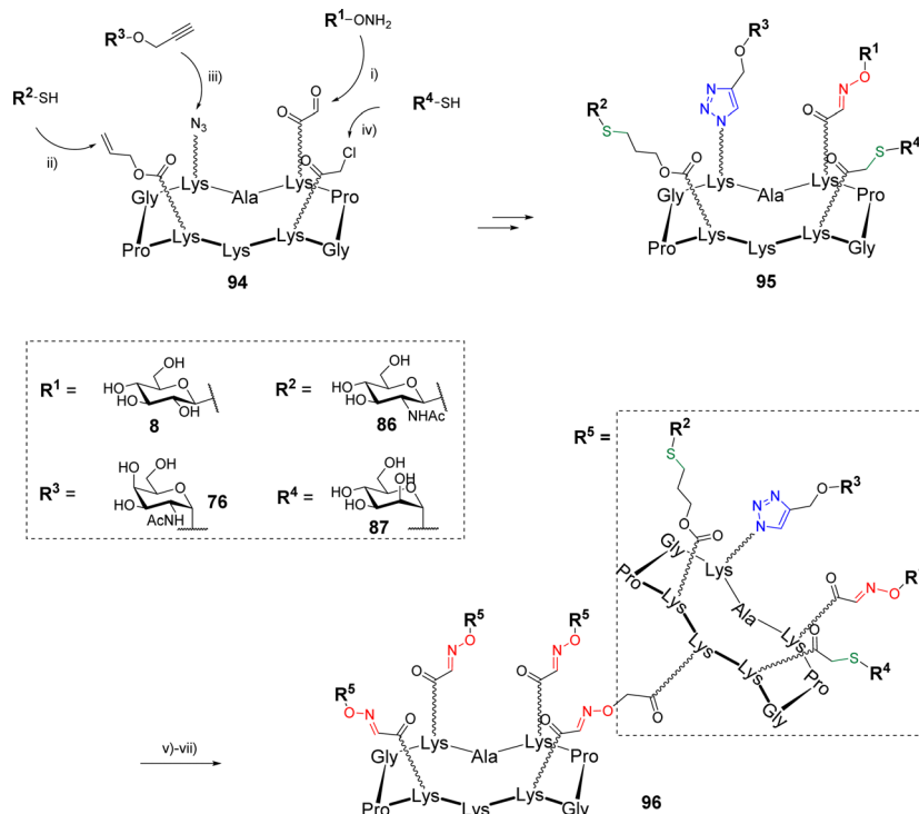
Scheme 19 Sequential one-pot synthesis of the heterovalent glycocluster 95 using four conjugation strategies and assembly of the glycodendrimer 96 . Reagents and conditions : (i) 0.1% TFA in \text{H}_2\text{O} , r.t., 30 min; (ii) DPAP, DMF/ \text{H}_2\text{O} , irradiation 365 nm, r.t., 30 min; (iii) \text{CuSO}_4 , THPTA, sodium ascorbate, DMF/PBS (1:1, pH 7.4), r.t., 1 h; (iv) KI, DMF/ \text{H}_2\text{O} (1:1), DIPEA, r.t., 1 h; 47% over four steps; (v) N -succinimidyl (Boc-aminoxy)acetate, DIPEA, DMF; (vi) 50% TFA in \text{CH}_2\text{Cl}_2 , r.t., 30 min, 93% over two steps; (vii) 51 , 0.1% TFA in \text{H}_2\text{O} , 37 °C, 30 min, 87%.
