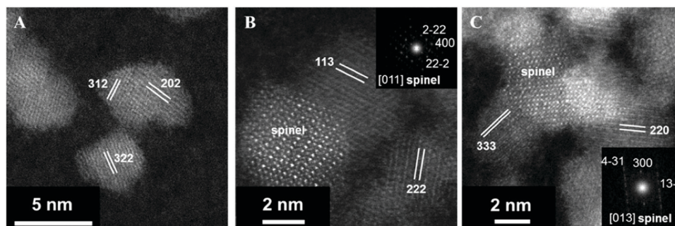
Fig. 39 High-resolution images of spinel-type CoV 2-x Fe x O 4 ( x = 0-2 ) nanoparticles: (A) CoFe 2 O 4 , (B) CoFeVO 4 , and (C) CoV 2 O 4 . Reproduced with permission from ref. 703. Copyright American Chemical Society 2018.
