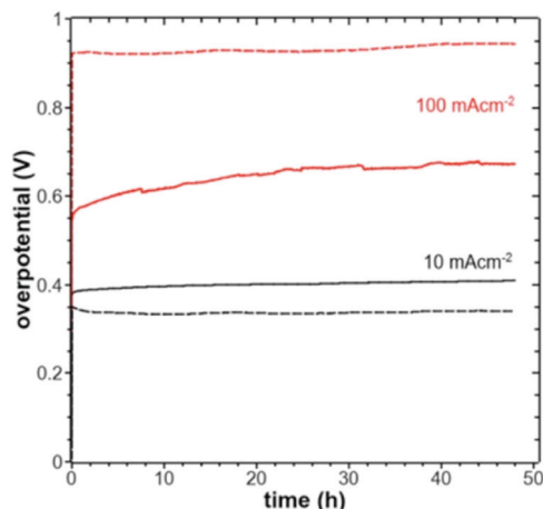
Fig. 38 Plot of the overpotential as a function of time at current densities of 10 mA cm -2 (black) and 100 mA cm -2 (red) measured in 1 M KOH for films deposited at 50 °C (dashed lines) and 103 °C (full lines). Reproduced with permission from ref. 733. Copyright American Chemical Society 2020.
