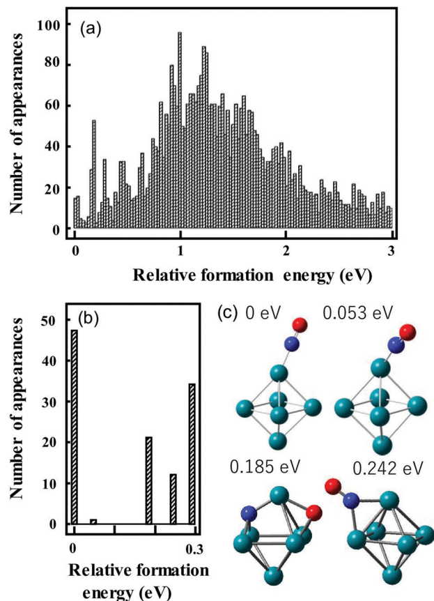
Fig. 3 Histograms of relative energies of \text{Rh}_6^+(\text{NO}) isomers calculated at the B3LYP/LANL2DZ (a) and B3LYP/sdd (b) levels of theory. For (b) all geometries in the [0,0.5 eV] interval in (a) were reoptimized. (c) Geometries of the four lowest-energy isomers in (b). Panel (a) reprinted with permission from ref. 97. Copyright (2021) Elsevier.
