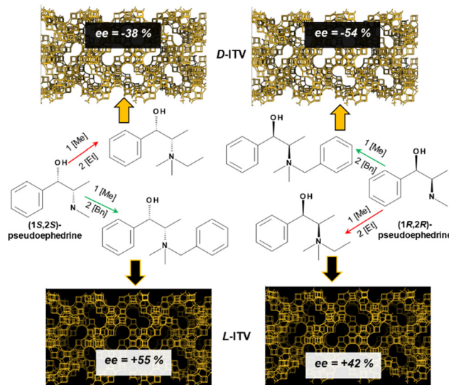
Fig. 1 Scheme of the synthetic route to the two enantiomorphic crystalline polymorphs of the -ITV framework ( P 4 32 and P 4 32 space groups) by using the two derivatives of the enantiomers of pseudoephedrine through GTM-3 (by attachment of an ethyl group, red-arrows routes) or GTM-4 (by attachment of a benzyl group, green-arrows routes). D/L notation is arbitrary and does not mean an actual absolute configuration of the zeolite.
