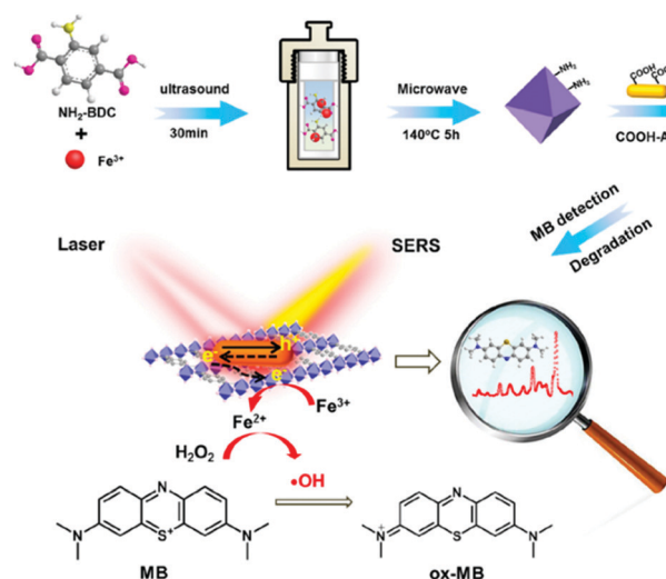
Fig. 9 Schematic diagram of the preparation of Au NRs/Fe-MOFs for methylene blue in situ catalytic degradation and SERS detection. Reproduced from ref. 138 with permission from American Chemical Society, copyright 2022.
