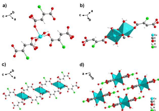
Fig. 43 Crystal structure of [\text{Cu}(\text{OOC}-\text{CH}=\text{Cl}-\text{COO})(\text{H}_2\text{O})_2] \cdot \text{H}_2\text{O} showing: (a) the coordination environment of Cu 2+ , (b) the dinuclear building unit with connecting chlorofumarate linkers, (c) one-dimensional ribbon extending along [001] and (d) the packing of ribbons viewed along [001]. Note: one oxygen atom of the carboxylate group neighbouring the CH moiety is disordered over two (split) positions. Graphics redrawn from the cif file (CSD-Refcode LEHJIS). 133
