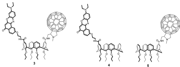
Fig. 1 Structures of the investigated compounds.
