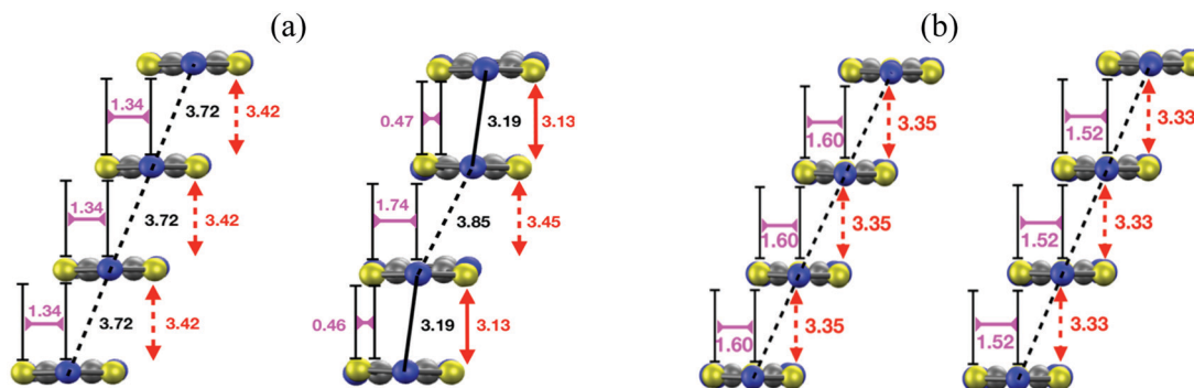
Fig. 15 (a) Side view of a \pi -stack of the (left) X-ray-resolved structure at 323 K of the HT polymorph of PDTA and (right) the optimized structure at 0 K. Although not shown in the images, the structure of the \pi -stacks of TTTA and NCBDTA is very similar to that of PDTA. (b) Side views of a \pi -stack of the (left) X-ray-resolved structure at 293 K of the HT polymorph of TDPDTA and (right) the optimized structure at 0 K. The black, red, purple and orange values shown in the image mark the distances between the nitrogen atoms of the S–N–S moieties of adjacent radicals, the interplanar distance between adjacent radicals and the degree of latitudinal and longitudinal slippage between adjacent radicals, respectively. Figures adapted with permission of ref. 114.
