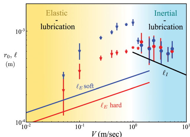
Fig. 6 r_0(V) is shown along with the calculated lateral scale \ell in both the elastic and inertial regime. Data for the soft impactor are shown in blue points while the data for the hard impactor are shown in red points; symbols indicate the means of impact as described in the legend of Fig. 2. Calculated \ell for the elastic (blue and red lines) and inertial (black line) regimes are plotted and labelled accordingly. The scaling regimes are illustrated using the background color – yellow corresponds to the elastic-lubrication stress balance, whereas cyan corresponds to the inertial-lubrication stress balance.
