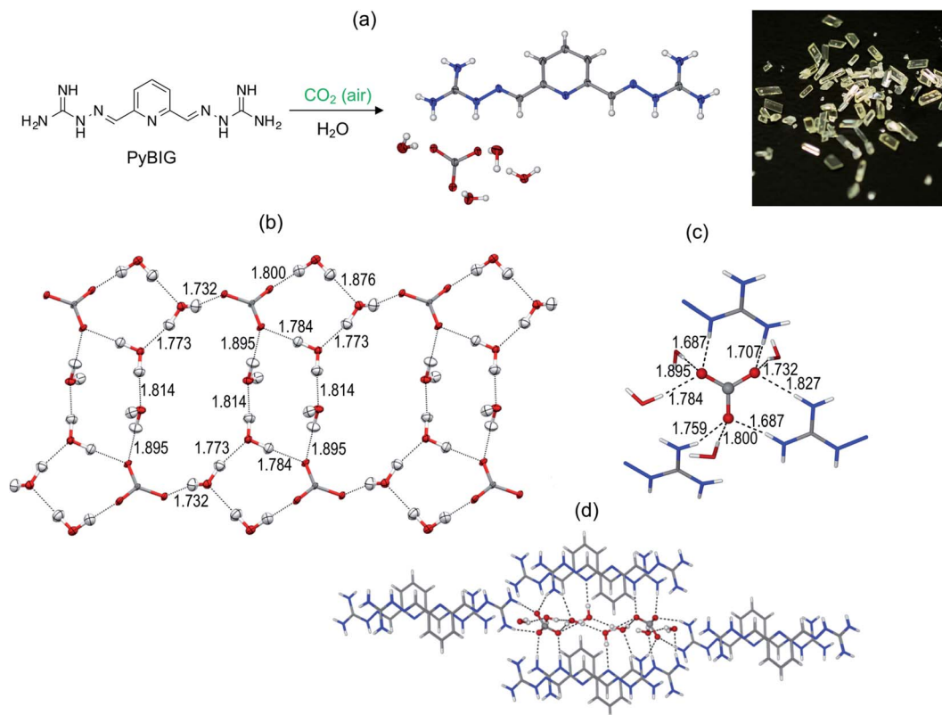
Fig. 8 DAC with PyBIG. (a) Crystallization of hydrated PyBIG carbonate from aqueous PyBIG and atmospheric \text{CO}_2 . (b) Extended carbonate–water clusters from the single-crystal neutron diffraction structure, with the hydrogen bond contacts in Å. (c) Carbonate binding site in the crystal, showing the hydrogen bond contacts (Å) from the guanidinium groups and water molecules. (d) Crystal packing consisting of cationic \text{PyBIGH}_2^{2+} stacks that flank the anionic [\text{CO}_3(\text{H}_2\text{O})_4]^{2-}_n clusters.
