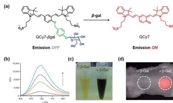
Fig. 2 (a) Fluorescence response of the NIR fluorescent probe QCy7- \beta gal to \beta -gal. Fluorescence response (b), absorbance response (c), and in vivo imaging (d) of QCy7- \beta gal.
