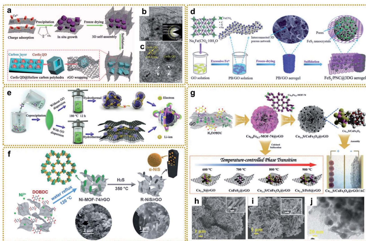
Fig. 8 (a) Schematic illustration for the fabrication procedure of (\text{Co}_9\text{S}_8 \text{ QD@HCP})\text{@rGO} sponge-like composites. (b) TEM and (c) HRTEM images of the (\text{Co}_9\text{S}_8 \text{ QD@HCP})\text{@rGO} . The inset in (b) is the SAED pattern of the composites. Reproduced with permission from ref. 150. Copyright 2017, Wiley-VCH. (d) Schematic illustration of the preparation process of a multi-scale \text{FeS}_2/\text{PNC@3DG} aerogel. Reproduced with permission from ref. 63. Copyright 2019, Royal Society of Chemistry. (e) Schematic illustration of the fabrication process of \text{ZnSnS}_3 and \text{ZnSnS}_3\text{@NG} nanocomposites. Reproduced with permission from ref. 151. Copyright 2020, American Chemical Society. (f) Schematic illustration of the synthesis procedure of the R-NiS/rGO from MOF precursors. Reproduced with permission from ref. 156. Copyright 2018, Royal Society of Chemistry. (g) Schematic diagram of the preparation of \text{Co}_{1-x}\text{S}/\text{CoFe}_2\text{O}_4\text{@rGO} and other temperature-controlled phases. (h) SEM images of \text{Co}_{0.8}\text{Fe}_{0.2}\text{-MOF-74@rGO} , and (i) SEM and (j) TEM images of \text{Co}_{1-x}\text{S}/\text{CoFe}_2\text{O}_4\text{@rGO} . Reproduced with permission from ref. 148. Copyright 2020, Wiley-VCH.
