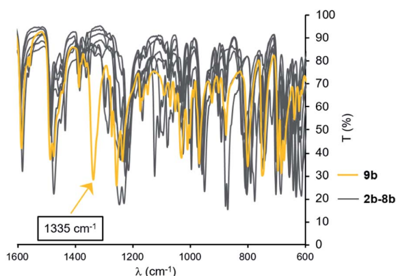
Fig. 3 IR spectra of BIPP complexes 2b–9b (ATR, 1600\text{--}600\text{ cm}^{-1} range).
