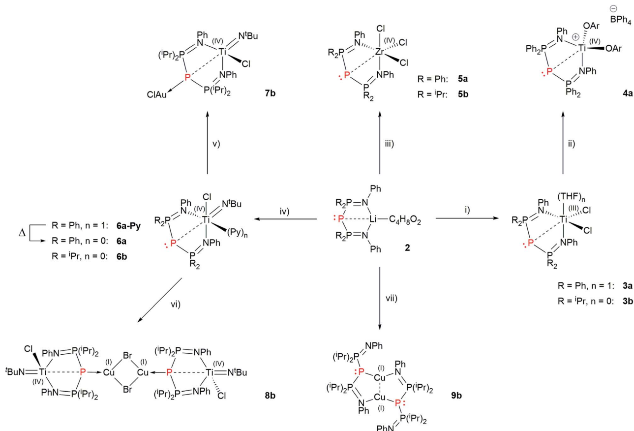
Scheme 6 Synthesis of group 4 and coinage metal complexes of BIPP. Reagents and conditions: (i) 1 eq. [\text{TiCl}_3(\text{THF})_3] , THF; (ii) 1 eq. [\text{Cp}_2\text{Fe}][\text{BPh}_4] , 2 eq. \text{ArONa} ( \text{OAr} = 2,6\text{-dimethylphenolato} ); (iii) 1 eq. \text{ZrCl}_4 , toluene; (iv) 1 eq. [\text{TiCl}_2(\text{N}^t\text{Bu})(\text{Py})_3] , toluene; (v) 1 eq. [\text{Au}(\text{THT})\text{Cl}] , \text{CH}_2\text{Cl}_2 ; (vi) 1 eq. \text{CuBr} , \text{CH}_2\text{Cl}_2 ; (vii) 1 eq. \text{CuBr} , toluene. All reactions were conducted at room temperature (THT = tetrahydrothiophene).
