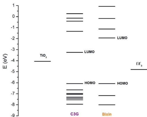
Fig. 1 Energy levels of the molecular orbitals of C3G and bixin. The energy levels of the redox couple \text{I}^-/\text{I}_3^- ( -4.9 eV) and of the conduction band of \text{TiO}_2 ( -4.0 eV) are also shown in the diagram.
