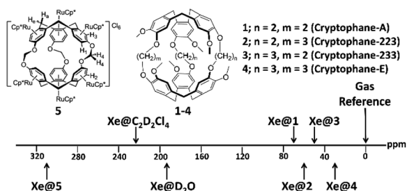
Fig. 1 Chemical structure and ^{129}\text{Xe} NMR chemical shifts of cryptophanes with varying alkoxy linker length in 1,1,2,2-tetrachloroethane- d_2 ( 1–4 ) 30 and of a cryptophane functionalized with six [ \eta^5\text{-C}_5\text{Me}_5 ] \text{Ru}^{\text{II}} moieties ( 5 ) 4 in \text{D}_2\text{O} .
