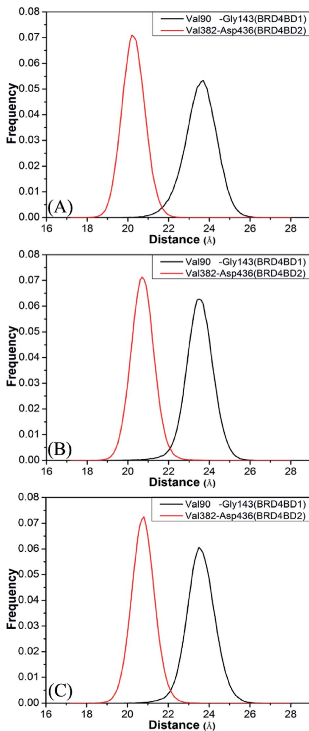
Fig. 5 Histogram distribution of C \alpha atoms of Val90 and Gly143 distance of BD1, histogram distribution of C \alpha atoms of Val382 and Asp436 distance of BD2: (A) the inhibitor 8NS, (B) the inhibitor 82Y, and (C) the inhibitor 837.
