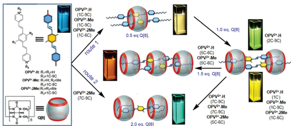
Scheme 1 Chemical structures of OPV^{2+} derivatives and Q[8] , and representation of Q[8] -based dynamic host-guest assemblies with multiple tunable fluorescence signals. Route 1: Q[8] concentration dependent host-guest interactions of 2 : 1, 2 : 2, 2 : 3, and 1 : 2 (guest/ Q[8] ); route 2: the formation of a U-shaped conformation of Q[8] with OPV^{2+} -2Me (7C-9C).
