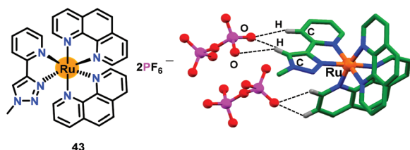
Fig. 20 Chemical drawing of chemosensor 43 and the crystal structure of 43 ·H 2 P 2 O 7 2- . Hydrogen atoms, except for those involved in H-bonding interactions, have been omitted for clarity. Adapted from ref. 66.
