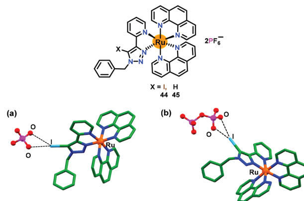
Fig. 21 Chemical drawings of chemosensors 44 and 45 . Crystal structures of (a) 44 ·H 2 PO 4 - and (b) 45 ·HP 2 O 7 3- complexes. Adapted from ref. 67.
