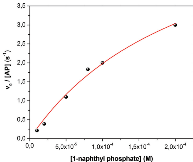
Fig. 2 Effect of 1-naphthyl phosphate concentration on the initial reaction rate ( v_0 ) of 1-naphthyl phosphate hydrolysis catalyzed by AP in buffer solution at 35 °C. [AP] = 1 \times 10^{-7} M. [buffer] = 0.01 M, pH = 10. The solid line represents the fit according to eqn (1).
