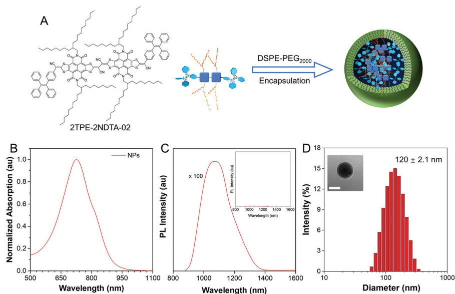
Fig. 1 (A) Schematic illustrations of fabrication of TN NPs by encapsulating DSPE-PEG 2000 with 2TPE-2NDTA-02. (B) Normalized absorption spectrum of TN NPs. (C) PL spectra of TN NPs. Concentration: 100 \mu\text{M} (based on TN); \lambda_{\text{ex}} = 820 nm. (D) DLS histogram and TEM image of TN NPs. Scale bar: 100 nm.
