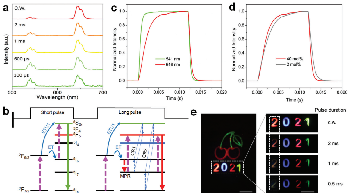
Fig. 7 (a) Upconversion emission spectra of \text{NaYF}_4\text{:Ho(40 mol\%)}\text{:NaYF}_4\text{:Yb(60 mol\%)}\text{:NaYF}_4 core–shell–shell nanoparticles under pulsed 980 nm excitation with a tuning of the pulse duration. (b) Schematic of the possible processes for the reduction of the red upconversion under non-steady state excitation. (c) Time-dependent emission profiles of \text{Ho}^{3+} at 541 and 646 nm of (a) sample under 980 nm irradiation with a pulse duration of 12 ms (50 Hz). (d) A comparison of the time-dependent red upconversion emission profiles from the (a) sample and \text{NaYF}_4\text{:Yb/Ho(20/2 mol\%)}\text{:NaYF}_4 core–shell nanoparticles. (e) Schematic of decoding the concealed information on the cherry pattern under pulsed 980 nm irradiation (right panels) in which only the initial number "2" shows a color change with reducing the pulse duration. Scale bars, 0.5 cm.
