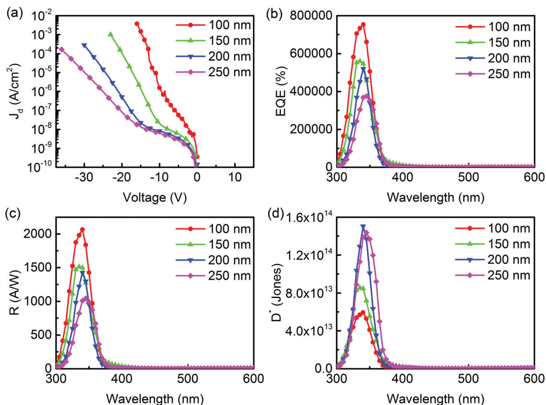
Fig. 4 (a) J_d , (b) EQE, (c) R , and (d) D^* characteristics of the fabricated UV PM-type OPDs with different active layer thicknesses. The device structure is ITO/TAPC: C_{60}(50:1, 100\text{ nm}, 150\text{ nm}, 200\text{ nm}, 250\text{ nm})/\text{Al} (100 nm).
