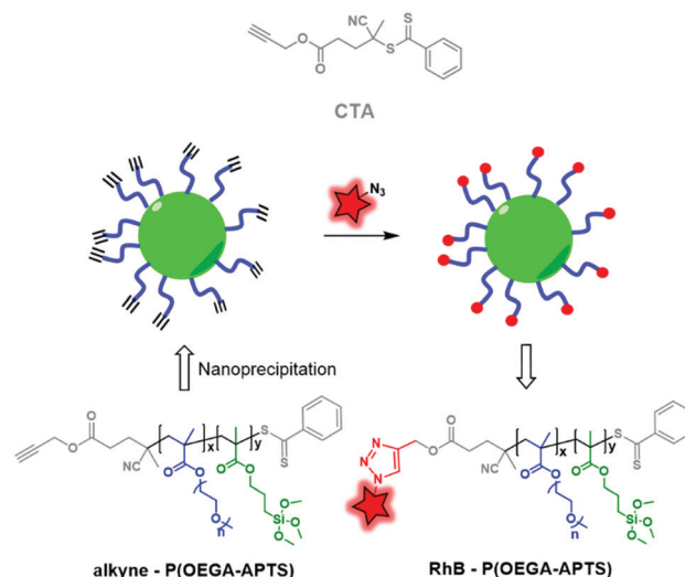
Fig. 32 P(POEGA-APTS) BCP obtained by RAFT polymerization using a clickable CTA, allowing labeling by RhB-azide.
