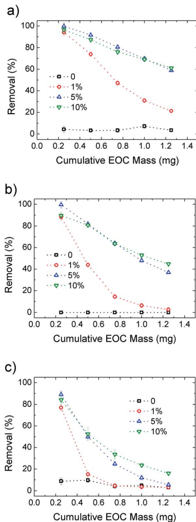
Fig. 9 Removal efficiency for Ciprofloxacin (a), OFLOX (b) and RhB (c) for PES and increasing GO loading in HF-GO. The cumulative initial mass is obtained with fixed concentration ( 5 \text{ mg L}^{-1} ) and flow ( 15 \text{ mL min}^{-1} ). Details are reported in Fig. S10. The curves for HF-GOe filters are shown in Fig. S11, ESI†
