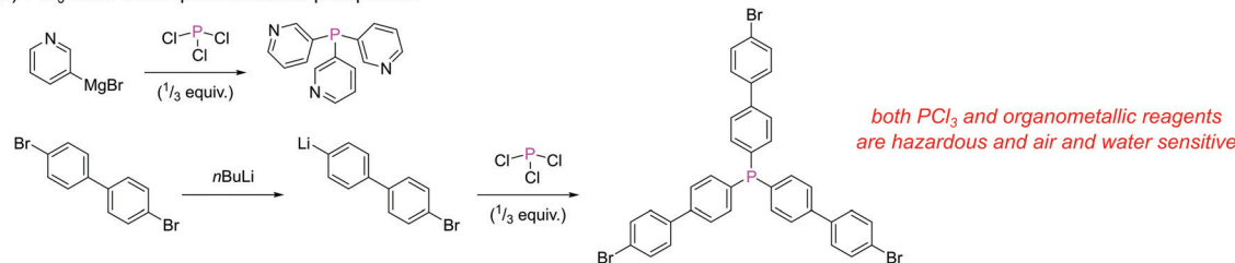
(c) nucleophilic sources of phosphorus
