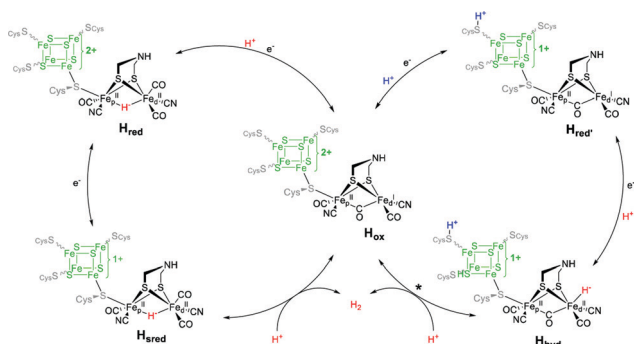
Fig. 20 Shortened catalytic cycle A from Fig. 3.11 and secondary cycle B, which is based on bridging hydrides. Red protons: catalytic PTP, blue proton: accessory PTP. * H_{ox}H might be involved in this conversion.
