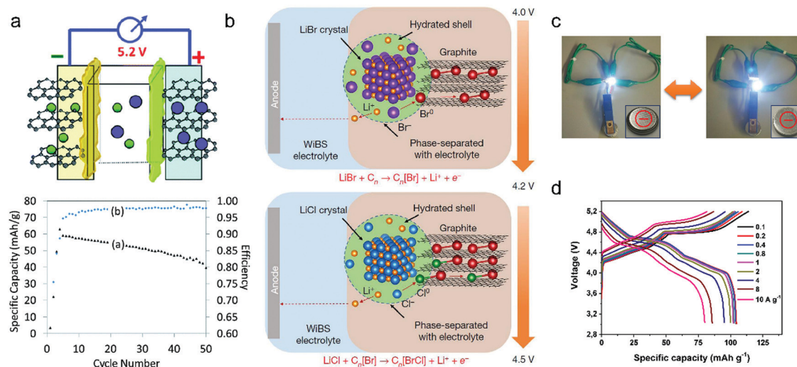
Fig. 25 (a) Schematic illustration of a dual-graphite intercalation cell and its electrochemical performance. Reproduced from ref. 206 with permission from The Royal Society of Chemistry. (b) Schematic of the conversion–intercalation mechanism occurring in the composite graphite cathode during its oxidation in the water-in-bisalt aqueous-gel electrolyte. The two-stage reactions involve the oxidation of \text{Br}^- (about 4.0\text{ V} ) and \text{Cl}^- (about 4.2\text{ V} ) and their subsequent intercalation into the graphitic structure. The discharge is a complete reversal of the charge process. Reproduced from ref. 172 with permission from Springer Nature. (c) Powering a white light-emitting diode by the polarity-switchable symmetric graphite battery from both directions. Reproduced from ref. 376 with permission from Wiley-VCH. (d) Rate performance of the Li-ion pseudocapacitor in a voltage window of 3\text{--}5.2\text{ V} . Reproduced from ref. 163 with permission from Wiley-VCH.
