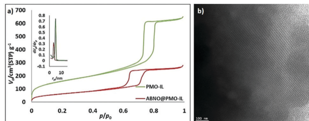
Fig. 2 (a) \text{N}_2 adsorption-desorption isotherms of all materials including PMO-IL and ABNO@PMO-IL-Cl and inset BJH pore size distribution. V_d refers to the volume of adsorbed nitrogen in the pores of the materials. (b) Side view TEM images of ABNO@PMO-IL-Cl. (Scale bar: 100 nm).
