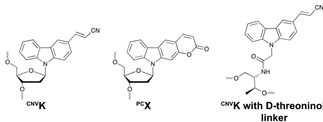
Fig. 6 Structure of 3-cyanovinylcarbazole ( ^{\text{CNVK}} ), pyranocarbazole ( ^{\text{PCX}} ) and 3-cyanovinylcarbazole with D-threoinol linker.
