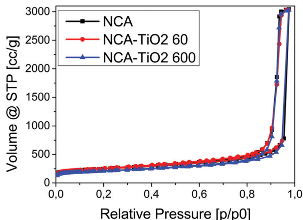
Fig. 3 Low temperature nitrogen adsorption-desorption isotherms.
