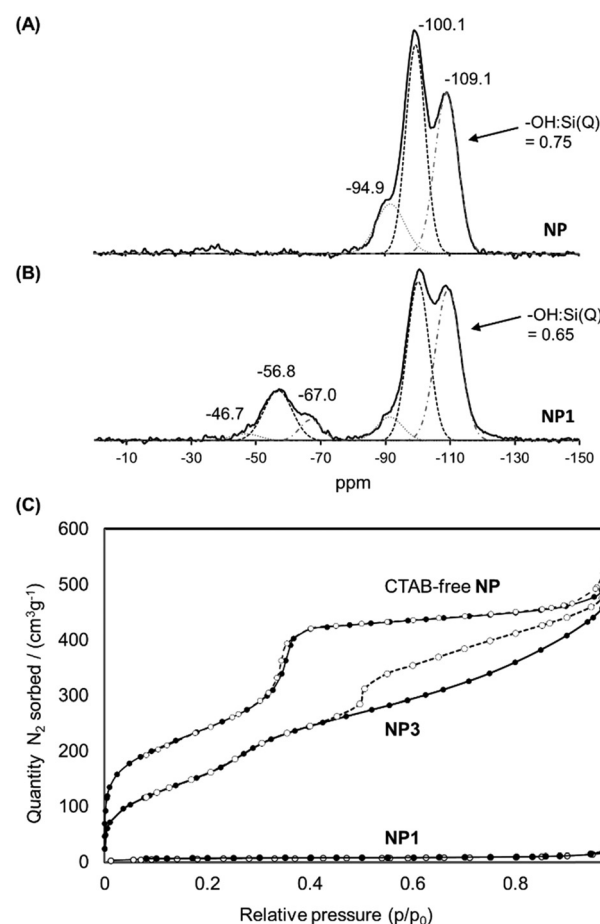
Fig. 5 Solid state ^{29}\text{Si} NMR spectra of NP (A) and NP1 (B). (C) Isotherms of CTAB-free NP , NP1 and NP3 obtained by nitrogen sorption analyses.
