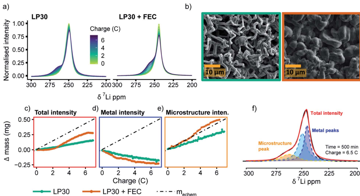
Fig. 2 (a) In situ NMR spectra obtained under a constant current of 0.5\text{ mA cm}^{-2} in LP30 and LP30 + FEC. (b) SEM images of the microstructures formed on applying a 0.5\text{ mA cm}^{-2} constant current in LP30 (left) and LP30 + FEC (right). (c) The total integrated intensity detected by NMR converted into mass change (mg) for a constant current of 0.5\text{ mA cm}^{-2} in LP30 (green) and LP30 + FEC (orange). The dashed line indicates m_{\text{echem}} , the mass deposited calculated based on the electrochemistry. A total of 6.5C of charge was passed, which corresponds to roughly 3.5\text{ mA h cm}^{-2} . (d and e) The integrated intensity of the deconvoluted metal peaks and microstructural peak converted into the change in mass, \Delta mass (mg). (f) An example of how the spectra for the LP30 electrolyte were deconvoluted into two overlapping metal peaks and one microstructural peak.
