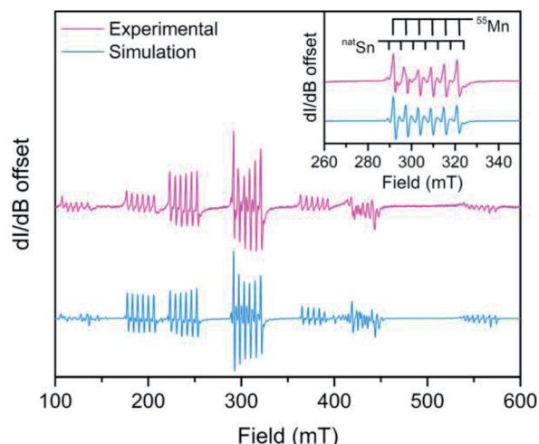
Fig. 4 Overlay of the experimental (pink) cw-EPR spectrum of 3 diluted in a polycrystalline sample of 7 ( \text{Mn} : \text{Zn} 1 : 20 ) and the simulation (light blue) at room temperature collected at X-band ( \nu = 9.6328\text{ GHz} ). Inset: a zoomed image of the intra-Kramers ( M_S = \pm\frac{1}{2} ) transition. The light blue spectrum was simulated using the following parameters: g_{\text{iso}} = 1.9933(2) , S = \frac{5}{2} , A_{\text{iso}}(^{55}\text{Mn}, I = \frac{5}{2}) = 164(2)\text{ MHz} , A_{\text{iso}}(^{\text{nat}}\text{Sn}, I = \frac{1}{2}) = 141(3)\text{ MHz} , D = 0.0939(4)\text{ cm}^{-1} .
