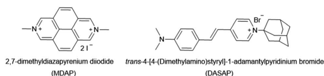
Fig. 6 Chemical structures of MDAP and DASAP.
