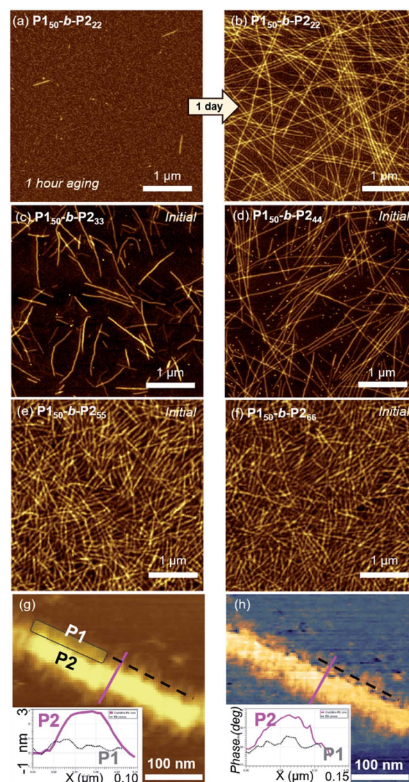
Fig. 2 AFM images obtained from 1 g L -1 chloroform solutions of (a) P1 50 -b-P2 22 after 1 h, and (b) after 1 d aging at 25 °C. (c) P1 50 -b-P2 33 , (d) P1 50 -b-P2 44 , (e) P1 50 -b-P2 55 , and (f) P1 50 -b-P2 66 without aging. The higher magnification of (g) height, and (h) phase images of the 1D nanofibers from P1 50 -b-P2 55 .
