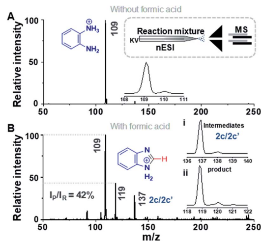
Fig. 1 Microdroplet synthesis of benzimidazole. (A) Mass spectrum of PDA in methanol without addition of formic acid. Insets show the isotopic distribution of the peak at m/z 109 and a schematic illustration of the setup. (B) Mass spectrum of PDA with FA at 1 : 1 molar ratio in methanol. Insets show the isotopic distributions of the peaks at (i) m/z 137 and (ii) m/z 119. I_P and I_R refer to the intensity of signals for product and reactant, respectively.
