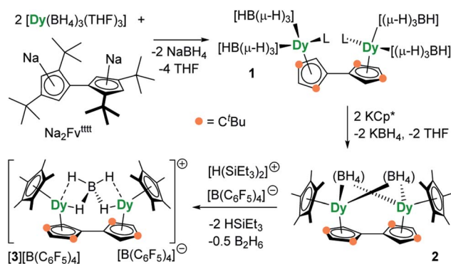
Scheme 1 Synthesis of compounds 1 , 2 and [\mathbf{3}][\text{B}(\text{C}_6\text{F}_5)_4] (L = THF).
