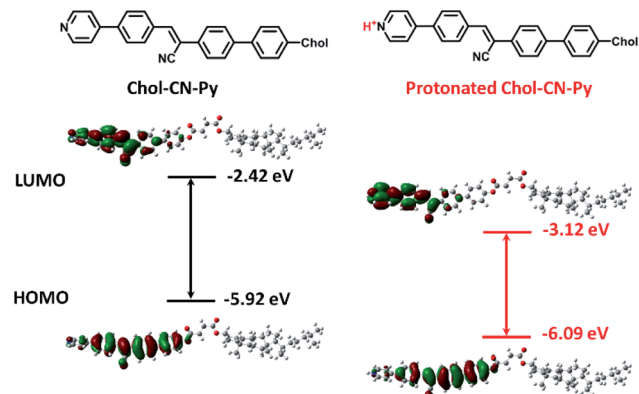
Fig. 4 The molecular structures and frontier molecular orbitals (including HOMO and LUMO energy levels) of Chol-CN-Py and protonated Chol-CN-Py.
