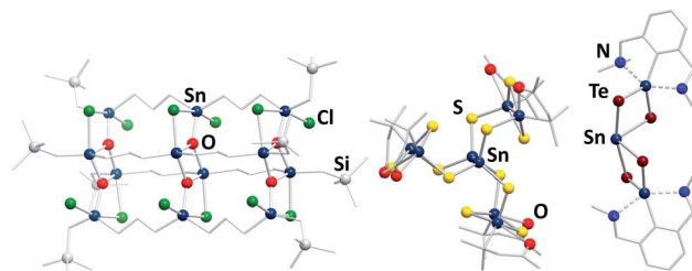
Fig. 3 From left: molecular structures of [\{\text{R}(\text{SnCl}(\text{CH}_2)_3\text{SnCl}(\text{CH}_2)_3\text{SnClRO}_3\}_4] ( \text{R} = \text{CH}_2\text{SiMe}_3 ), 46 [(\text{R}(\text{Sn}^{\text{IV}})_6\text{Sn}^{\text{III}})\text{S}_{12}] ( \text{R} = \text{CMe}_2\text{CH}_2\text{CO}(\text{Me}) ), 60 and [(\text{R}(\text{Sn})_2\text{SnTe}_4)] ( \text{R} = 2,6\text{-(Me}_2\text{NCH}_2)_2\text{C}_6\text{H}_3 ). 62
